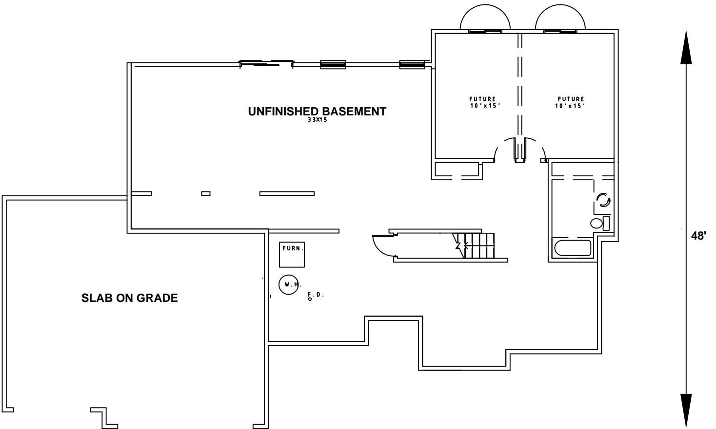
FOUNDATION PLAN
