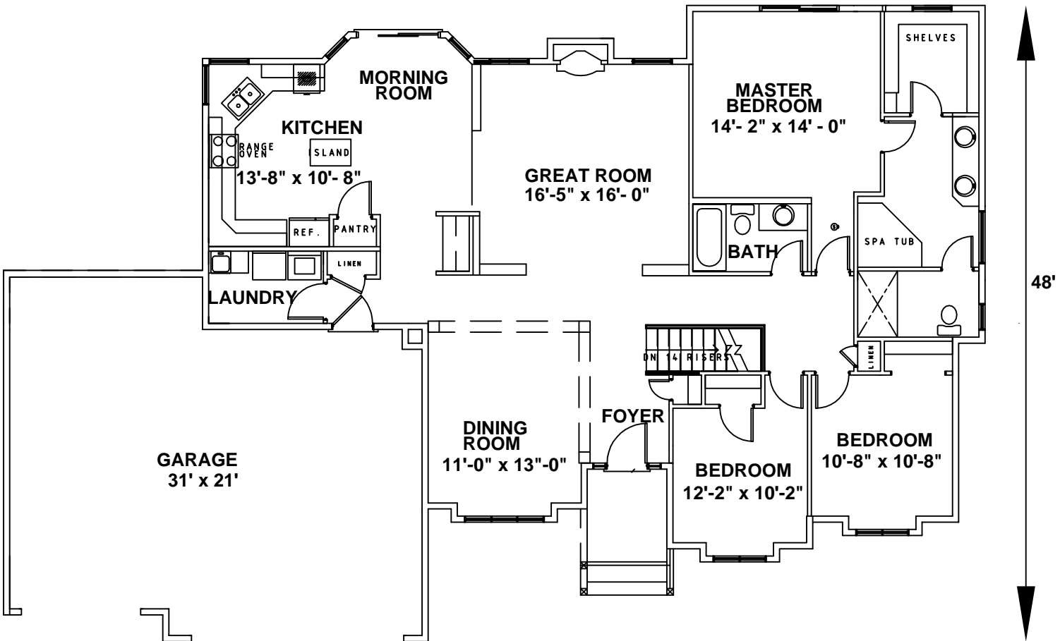
FLOOR PLAN
