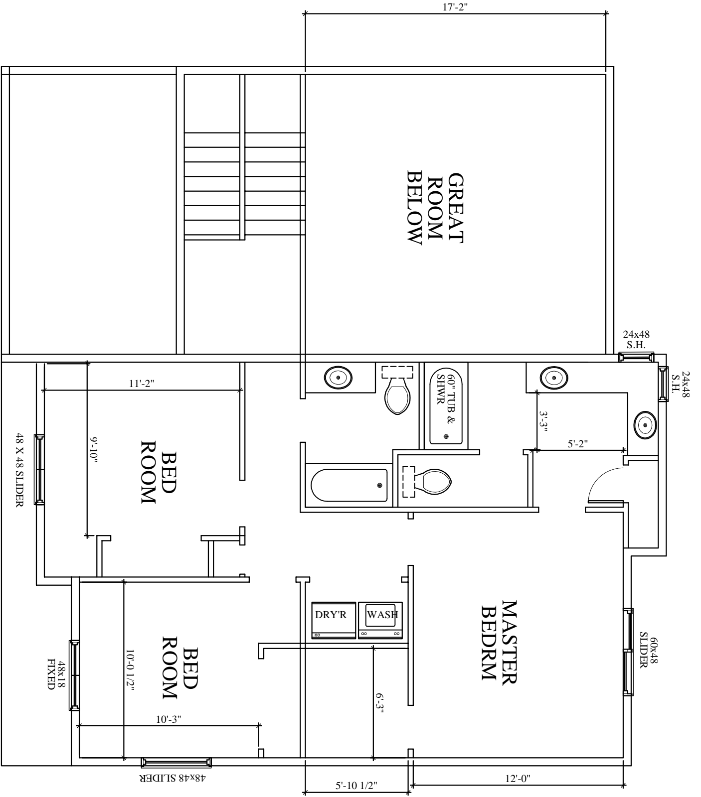
UPPER FLOOR 802 SQFT
